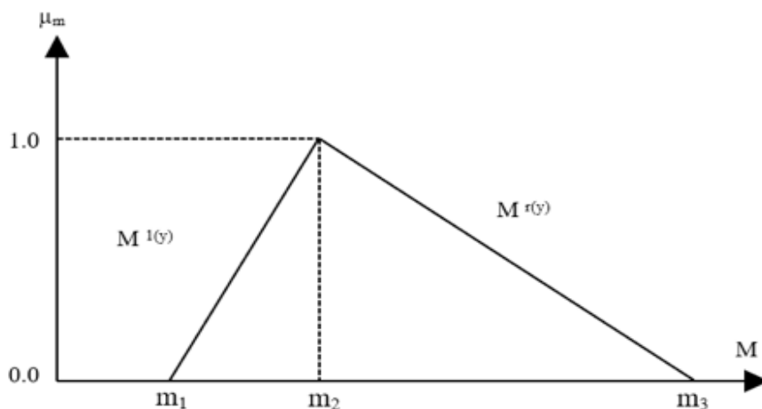
Figure 1: Triangular fuzzy values.
